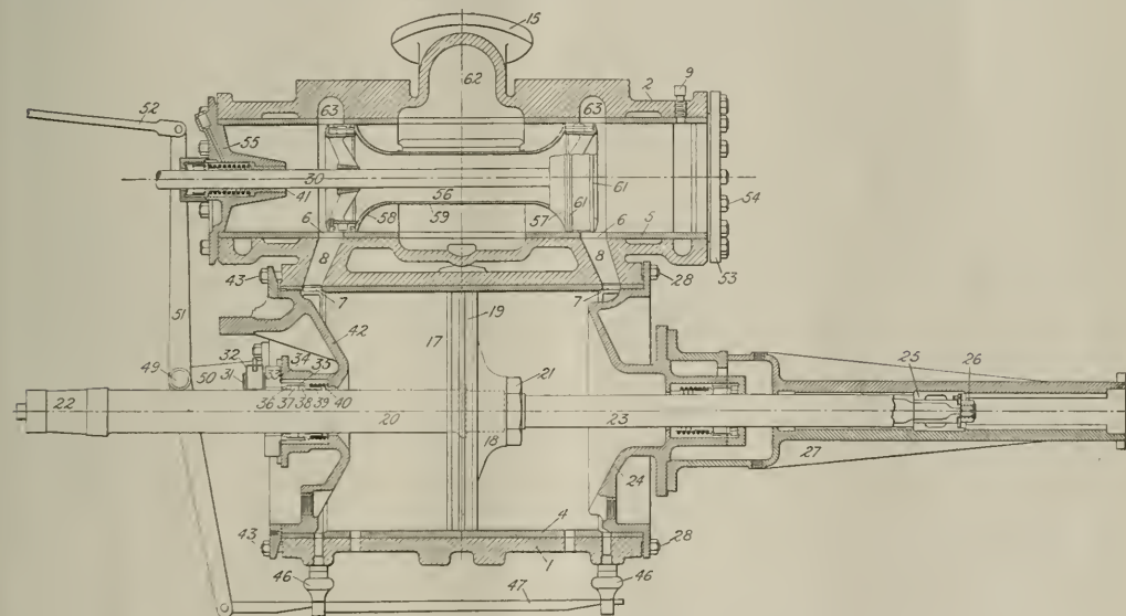
LONGITUDINAL SECTION OF CYLINDER AND STEAM CHEST
